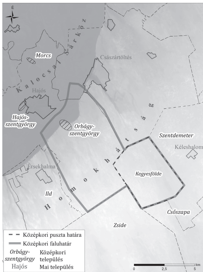
Figure 2 Topographical map of the area around Orbágy-szentgyörgy (Created by István Pánya)
