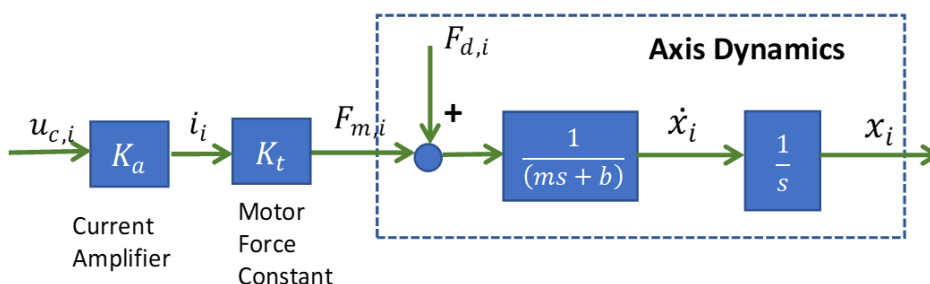
Figure 1. Block diagram of linear drive machine tool [1]
